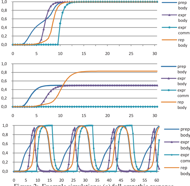
Figure 2: Example simulations: (a) full empathic response, (b) reduced emotion integration, (c) enhanced sensitivity
