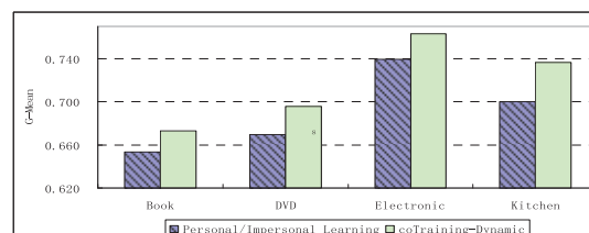
Figure 4: Comparison with the State-of-the-Art [Li et al. 2010]
