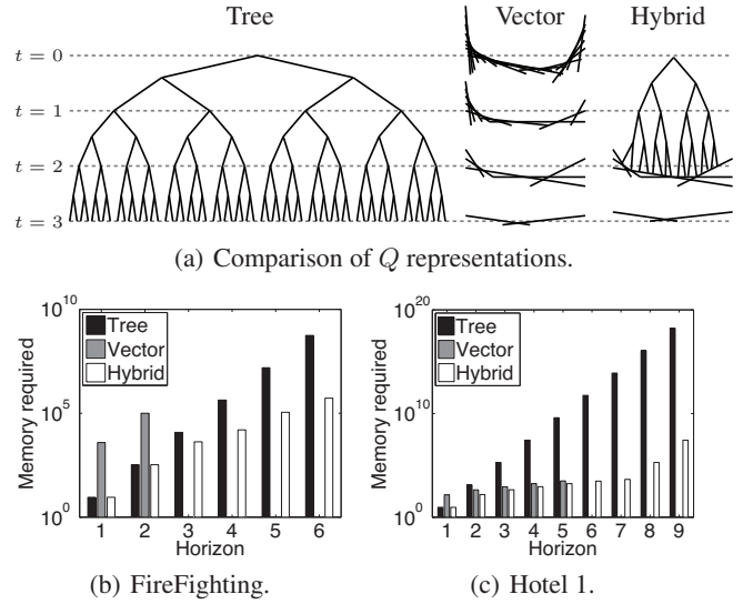
Figure 2: Hybrid heuristic representations. (a) Comparison of different representations. (b), (c) The number of real numbers stored for different representations of Q_{BG} .
