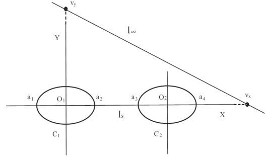
Figure 1: Two conics \mathbf{C}_1 and \mathbf{C}_2 have a common axis of symmetry \mathbf{l}_s . The line at infinity \mathbf{l}_\infty intersects the x-axis and y-axis with the point \mathbf{v}_x and \mathbf{v}_y .
