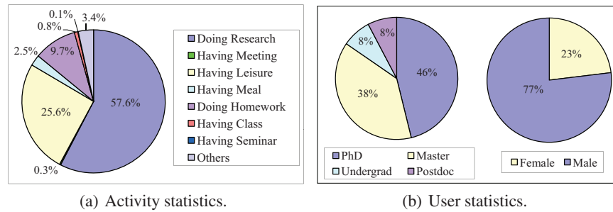
Figure 2: Data statistics.
