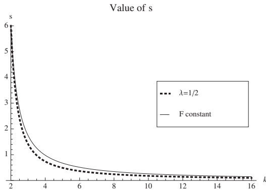
Figure 5: Maximum admissible value of s for varying number of categories k such that coverage remains 1/2 and fitness remains constant (equal to the fitness for k = 2 ).
