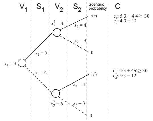
Figure 2: Policy tree for the sampled SCSP in Example 2
