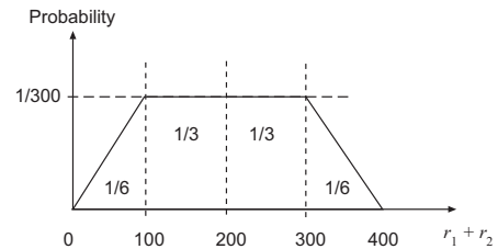
Figure 3: Probability density function of the convolution of two independently non-identically distributed uniform random variables r_1 and r_2 .
