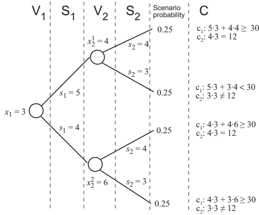
Figure 1: Policy tree for the SCSP in Example 1
