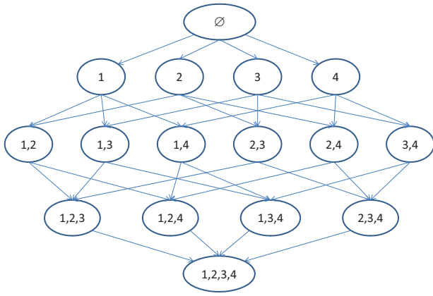
Figure 1: An order graph of four variables
