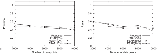
Figure 3: Accuracy of our algorithm and FSAP.
