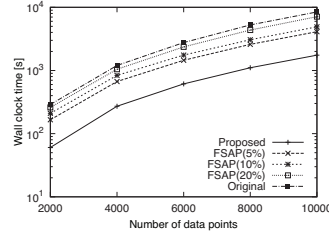
Figure 2: Scalability.
