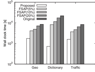
Figure 1: Clustering time.
