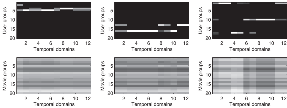
Figure 3: Some examples of user-group membership drift (upper row, the gray scales indicate membership proportions) and corresponding user-interest drift over movie groups (bottom row, gray scales indicate expected rating values in [1, 5] ).
