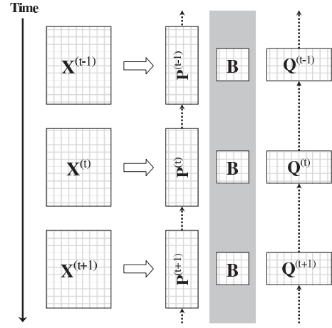
Figure 1: A framework for temporal-domain CF. Shaded rectangle means sharing and dotted arrows mean dependence.
