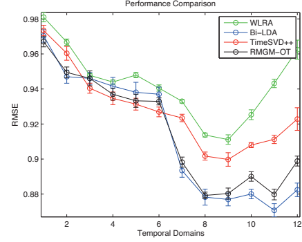
Figure 2: Performance comparison over temporal domains.
