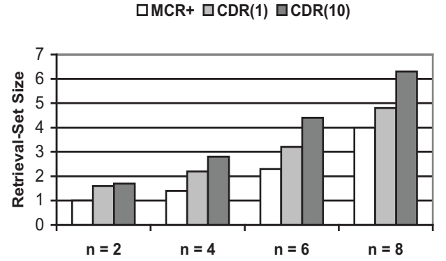
Figure 2. Average sizes of \text{MCR}^+ , \text{CDR}(1) , and \text{CDR}(10) retrieval sets for query sizes n = 2, 4, 6 , and 8 on the PC dataset.
