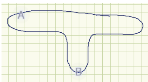
(a) a simple 'body'
