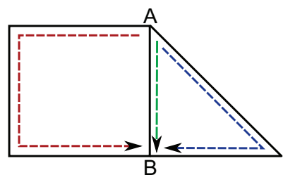
(a) a shared edge with three distinct paths
