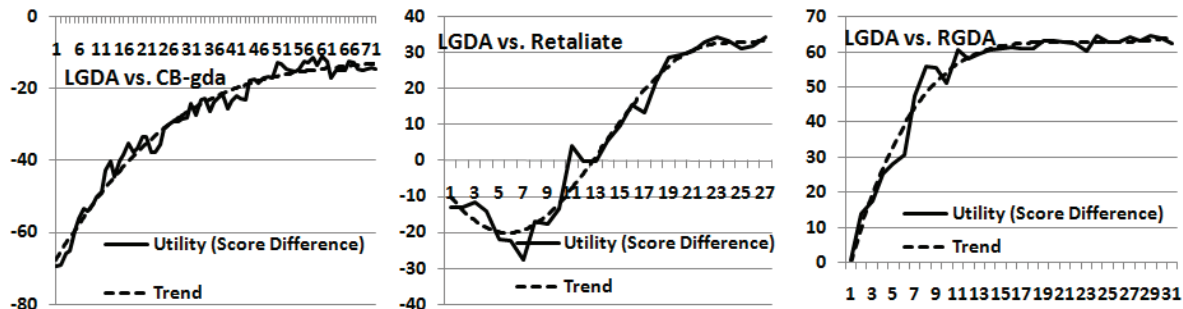
Figure 3: Results from Experiment 2: Average learning curves for comparing LGDA DOM performance vs. non-learning and ablated agents. The trend lines were generated using a polynomial fit to the raw curves.
