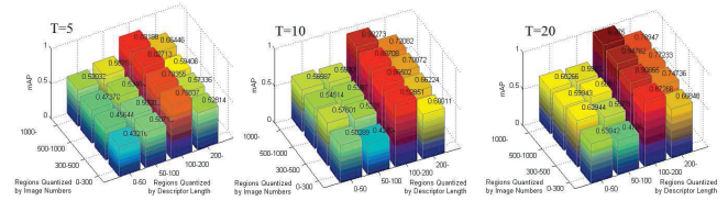
Figure 7: mAP variances in different regions, we draw two dimensional lattices to divided regions with respect to different image volumes and descriptor bits, then average the mAP for regions falling into each lattice.
