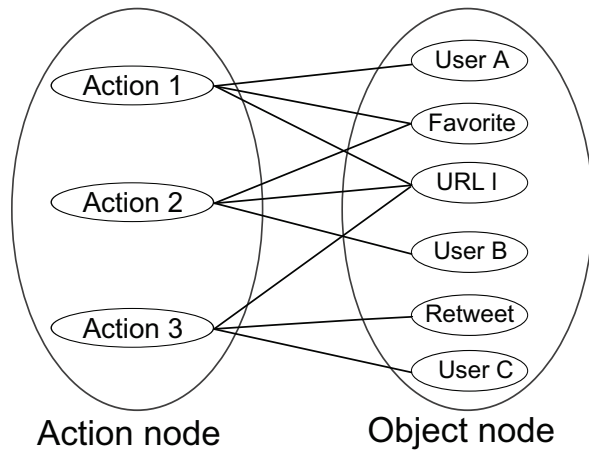
Figure 1: An example of ActionGraph representation.
