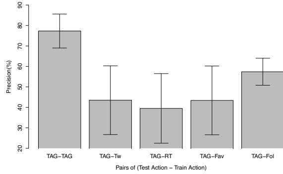
Figure 4: Predicting Delicious tagging by twitter actions.
