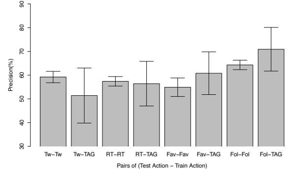
Figure 3: Predicting twitter actions by Delicious tagging.
