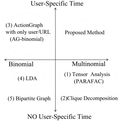
Figure 5: Baseline Methods.
