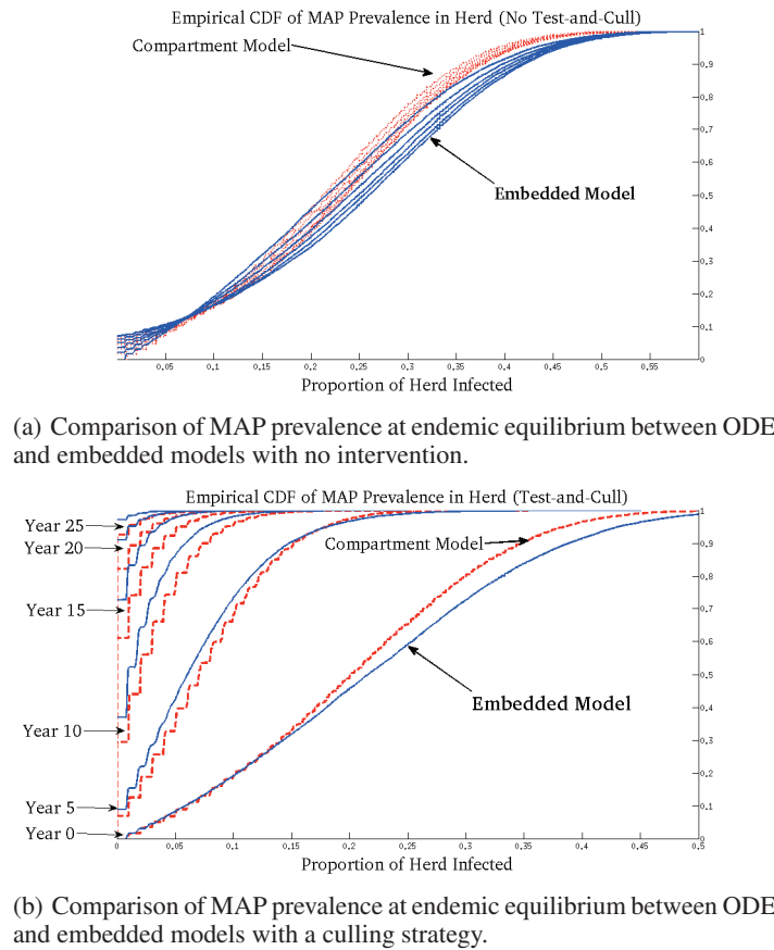
Figure 3: Results for experiments validating the Embedded model for MAP against the ODE based Coupled Model.
