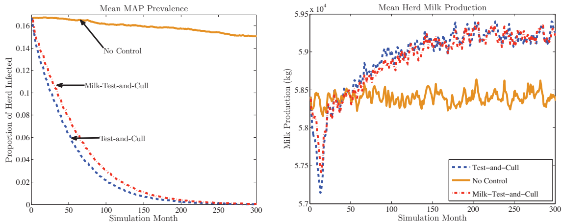
(a) Comparison of mean MAP prevalence over time between three control strategies. (b) Comparison of mean herd milk production over time between three control strategies.
