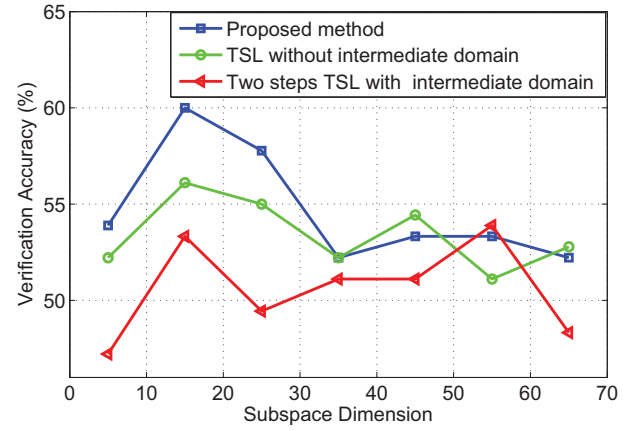
Figure 5: Verification accuracy vs. subspace dimensions.
