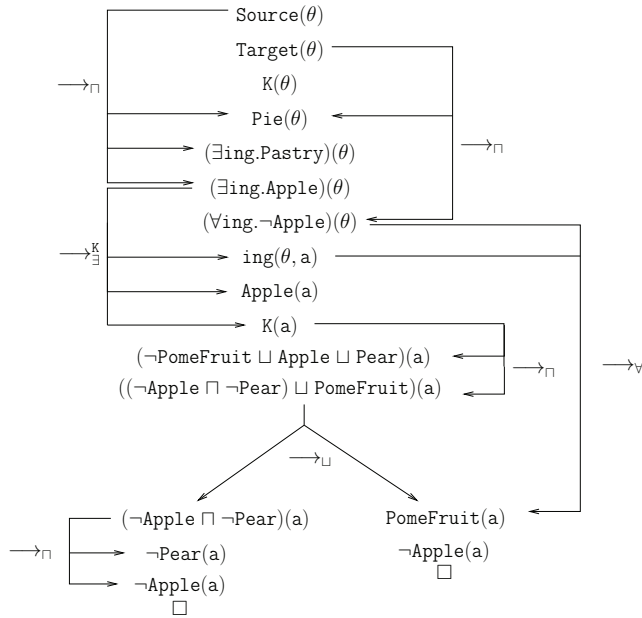
Figure 1: Application of the tableau method proving that the ABox \{\text{Source}(\theta), \text{Target}(\theta)\} is not satisfiable, given the TBox \{\top \sqsubseteq K\} (the order of application of rules has been chosen to make the example illustrative).
