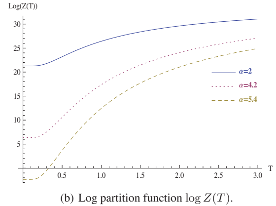
Figure 1: Average DOS (a) and log-partition function as a function of the temperature parameter T (b). The number of variables is n = 50 (see pdf for color version of figures).
