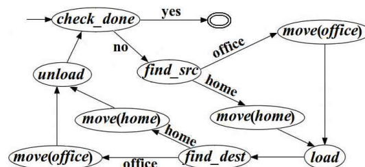
Figure 1: An example plan for the logistic problem
