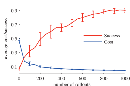
Figure 5: This figure shows the cost function of the table tennis task in simulation averaged over 10 runs with the error-bars indicating standard deviation. The red line represents the percentage of successful hits and the blue line the average cost.
