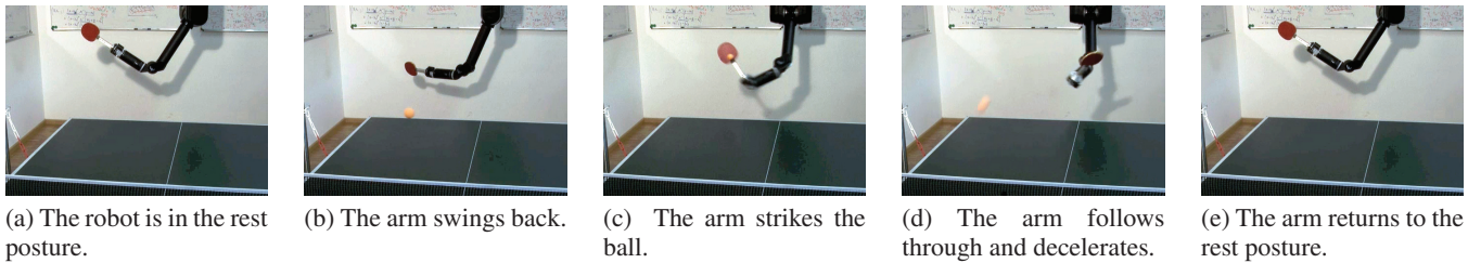
Figure 6: This figure shows a table tennis stroke on the real Barrett WAM.
