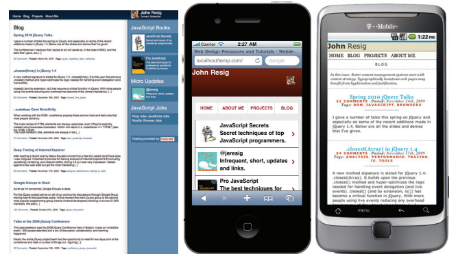
Figure 7: Flexible tree matching can be used to retarget Web pages designed for the desktop to mobile devices. Left : the original Web page. Right : the page automatically retargeted to two different mobile layouts.
