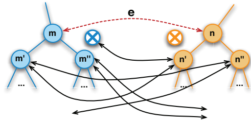
Figure 5: To bound c_a([m, n]; M) , observe that neither m' nor n' can induce an ancestry violation. Conversely, m'' is guaranteed to violate ancestry. No guarantee can be made for n'' . Therefore, the lower bound for c_a is w_a , and the upper bound is 2w_a .
