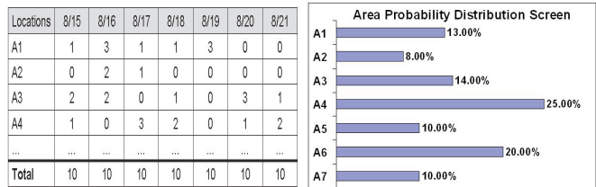
(a) Summary of sample schedule (b) Summary of area probability
