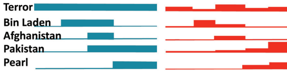
Figure 3: Activation patterns found by our algorithm for a chain connecting 9/11 to Daniel Pearl’s murder. Left: activation levels. Right: activation levels weighted by the influence (rescaled). For illustrative purposes, we show the result of the integer program (IP).
