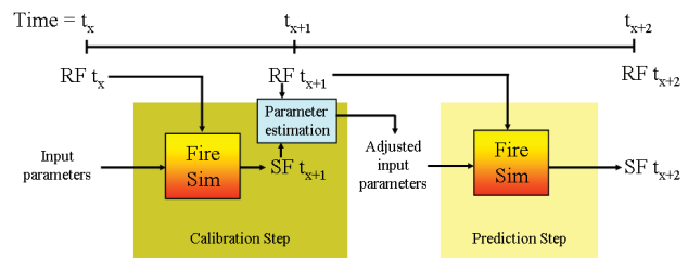
Figure 1: Two-stage fire prediction scheme.
