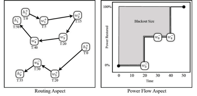
Figure 7: The Two Aspects of Power System Restoration.
