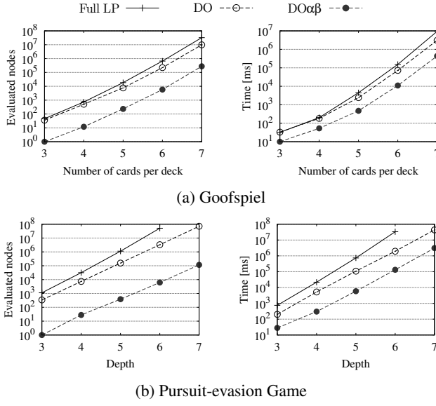
Figure 2: Comparison of evaluated nodes and running time for (2a) Goofspiel, and (2b) a pursuit-evasion game.
