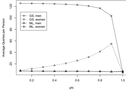
Figure 2: Average number of queries per person: n = 250 , 20 trials. Solid: proposers. Dashed: acceptors; Circles: GS-elastic, Triangles: RBH-PPGS-ML.
