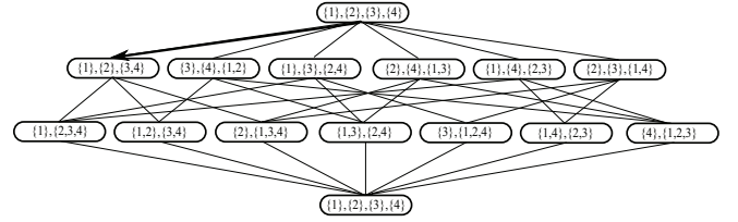
Figure 2: A diagram of the coalition structure graph for 4 agents. The downwards arrow shows the path followed by our approach.
