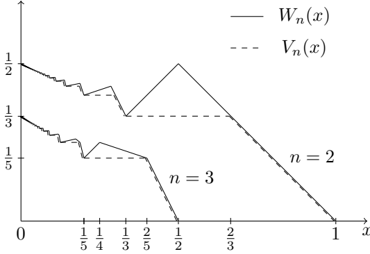
Figure 1: W_n(\cdot) and V_n(\cdot) for n = 2 and n = 3 .
