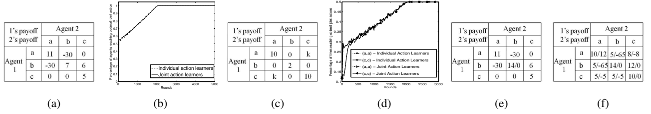
Figure 1: (a) The climbing game, (b) Percentage of agents reaching optimal joint action in climbing game, (c) The penalty game, (d) Percentage of agents reaching optimal joint actions in penalty game, (e) Partially stochastic climbing game ((b, b) yields the payoff of 14 or 0 with equal probability.), and (f) Fully stochastic climbing game (each joint action yields two different payoffs with equal probability.)
