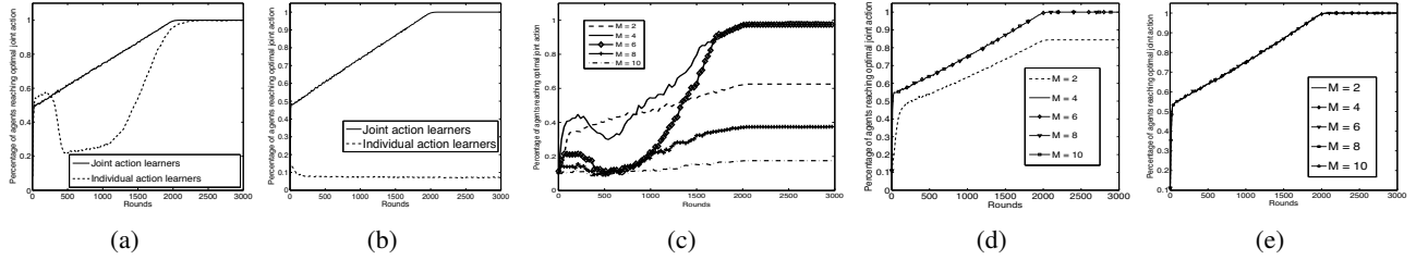
Figure 2: Percentage of agents coordinating on optimal joint action(s) in : (a) partially stochastic climbing game, (b) fully stochastic climbing game, (c) partially stochastic climbing game when M varies for IALs, (d) deterministic climbing game when M varies for IALs, and (e) fully stochastic climbing game when M varies for JALs (averaged over 500 times)
