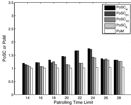
Fig. 2: PoM and PoSC under the Homogeneous Distribution.
