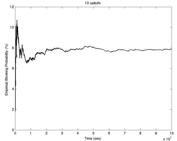
Figure 4: Blocking Probability of PD algorithm
