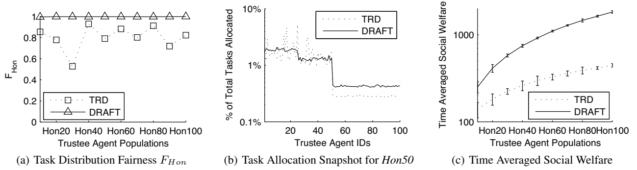
Figure 3: Comparing the Performance of the DRAFT Approach against the traditional accept-when-requested Approach.
