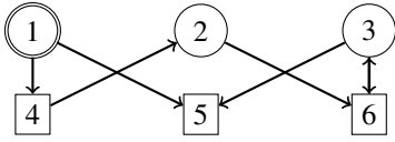
Figure 2: An instance of GG with 1 as the starting vertex.
