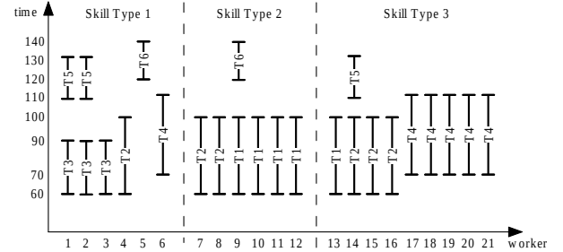
Figure 1: A feasible solution to the MAPTWTC instance.
