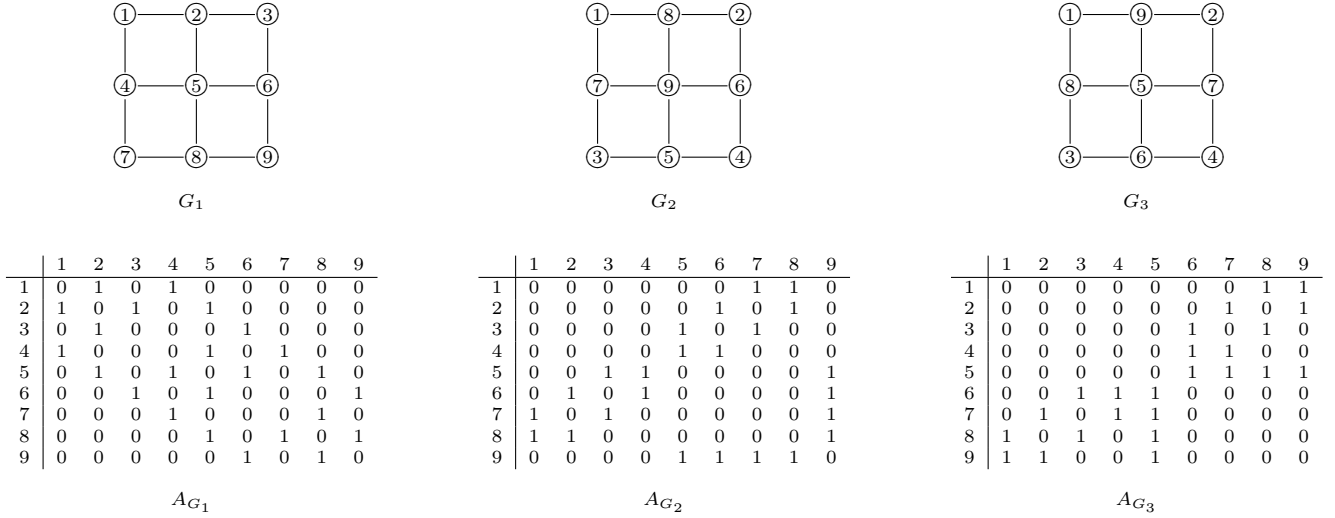
Figure 1: Three example graphs and their adjacency matrices
