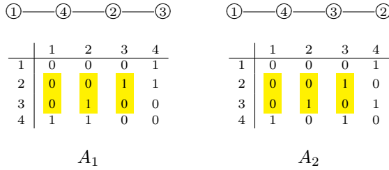
Figure 2: Graphs and adjacency matrices for Example 4.
