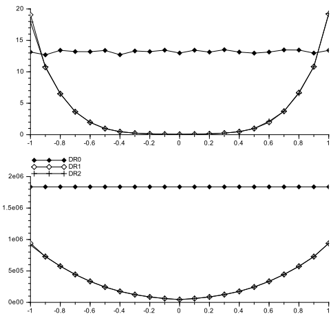
Figure 1: \alpha \in [-1, 1] , exec. time (s) (top), #subsol. (bottom)
