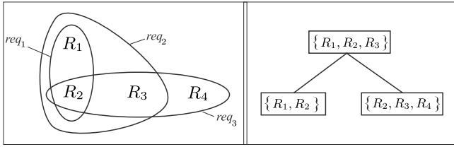
Figure 2: The hypergraph in Example 3.1, and a join tree for it.
