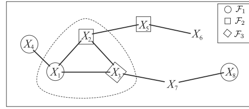
Figure 3: The (hyper)graph in Example 4.3
