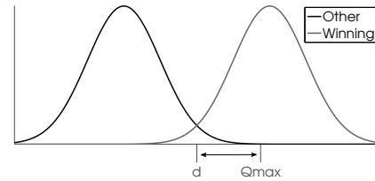
Figure 7: We gather statistics for the difference between d and Q_{max}
