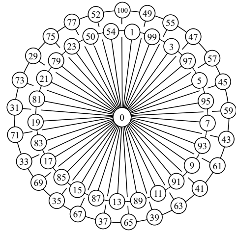
Figure 5: Double-wheel graph of size 25 ( DW_{25} ) with the graceful labeling generated by the proposed constructive procedure (case N is odd). This is the largest graceful double-wheel graph ever reported in the literature.
