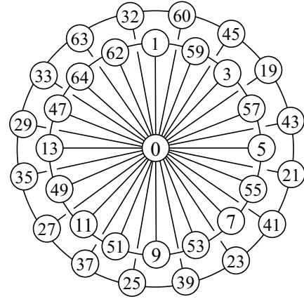
Figure 4: Double-wheel graph of size 16 ( DW_{16} ) with the graceful labeling generated by the proposed constructive procedure (case N is even).
