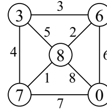
Figure 1: Example of a graceful graph. Each node is assigned a unique label from 0 to 8, where 8 is the number of edges. The label of an edge corresponds to the absolute difference of the labels of its endpoints and is unique among all 8 edges.
