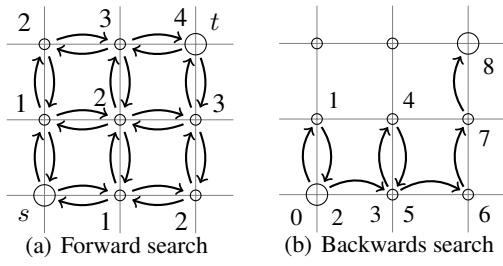
Figure 2: The first iteration of BTVS for solving a pathfinding problem from (0, 0) to (2, 2) with T = 9 in a 3 \times 3 grid
