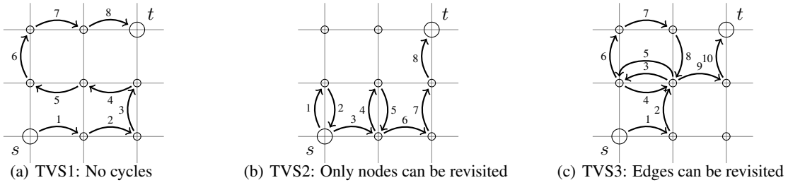
Figure 1: Solutions to the different TVS variants in a 3 \times 3 grid with T = 9
