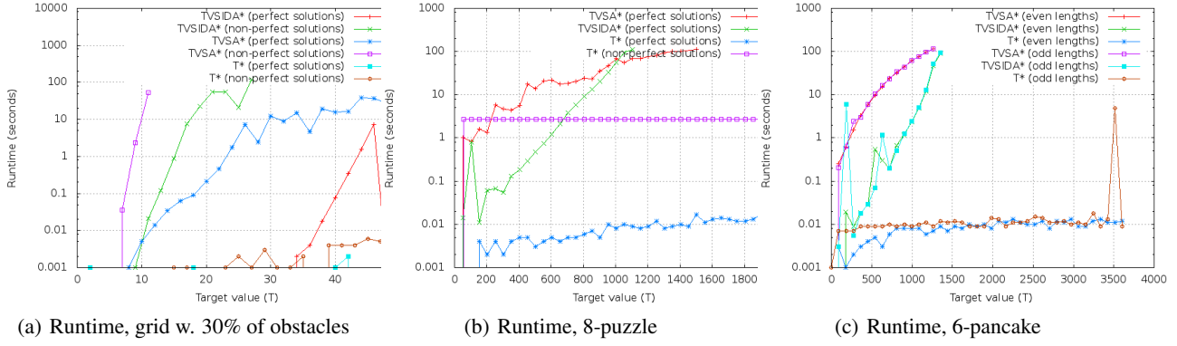
Figure 4: Average running time of all algorithms over 10 problems with different target values
