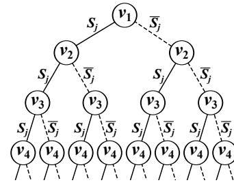
Figure 2: The space explored by Recursive Number Partitioning (RNP). Binary decision variables ( v_1, v_2, \dots, v_n ) correspond to individual numbers. Leaf nodes correspond to decompositions for which optimal solutions must be generated.
