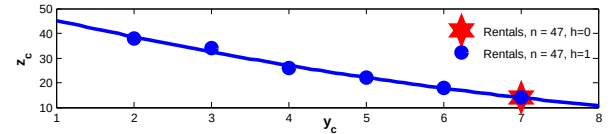
Figure 4: Pareto frontier for Scheduling with Rentals.
