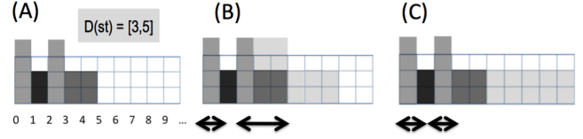
Figure 2: (A) Problem with 4 fixed activities and one activity of length 5 that can start from time 3 to 5. We assume D(y_c) = \{2\} , len = 3 and k = 0 . (B) Solution satisfying WEIGHTEDFOCUS with z_c = 4 . (C) Solution satisfying WEIGHTEDFOCUS with z_c = 2 .
