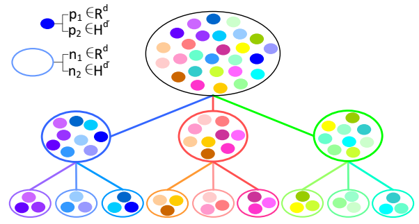
Figure 1: An example of hierarchical k -means tree with struct nodes. A solid dot represents a data point, while a hollow ellipse represents a data cluster which is a node in HKM tree. Each point has two representations: p_1 and p_2 , p_1 stands for the representation in original data space \mathbb{R}^d and p_2 stands for its representation in Hamming space \mathbb{H}^{d'} . Similarly, each node also has two representations: n_1 \in \mathbb{R}^d and n_2 \in \mathbb{H}^{d'} .
