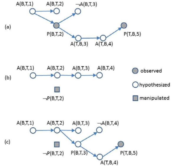
Figure 3: An example of three explanations given (a) two observed events, (b) two observed events followed by manipulation, and (c) two observed events, followed by manipulation, followed by a repeated observation of P(T, B, 5) . A \equiv Angry , P \equiv Punch , B = Bob and T = Tom .
