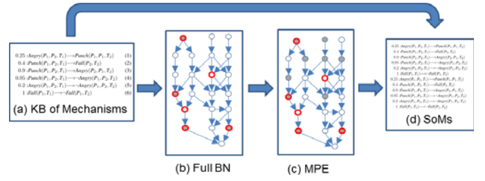
Figure 4: A high-level flow of our SoM algorithm.
