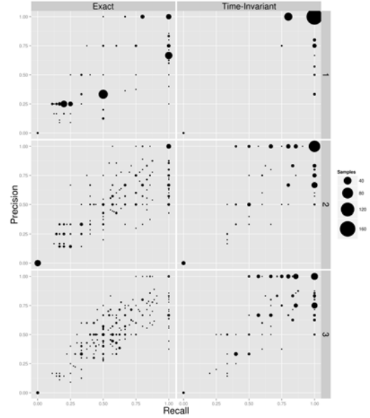
Figure 5: Precision-Recall for Exact Matches (left) and Time-Invariant matches (right) for 1,2, or 3 starting predicates (top, middle, and bottom).
