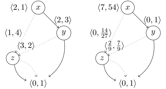
Figure 1: An e-SLDD _\star formula (left) and the corresponding \min_\star -reduced e-SLDD _\star formula (right). x, y and z are Boolean variables. A (resp. plain) edge corresponds to the assignment of the variable labeling its source to 0 (resp. 1).
