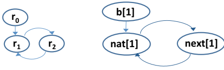
Figure 1: Activation (left) and argument (right) graphs of \mathcal{P}_3 .
