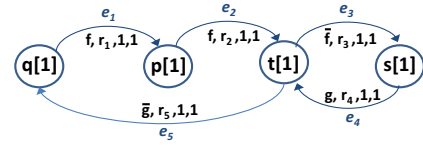
Figure 3: An example of a non-simple basic cycle.
