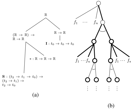
Figure 1: (a) The typed combinator S * I ( f(x) = x^2 over real values ( \mathbb{R} )) represented as a binary tree. (b) The space of all typed combinators represented as an infinitely deep AND/OR tree.
