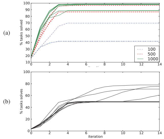
Figure 6: Learning curves from Boolean function learning experiments. (a) Learning curves for various frontier sizes on task set of circuit based Boolean functions. (b) 10 learning curves for frontier size of 2000 on a task set consisting of all Boolean functions of cardinality 3 or smaller. Note how most of the trajectories get stuck in a local minimum around 50%.
