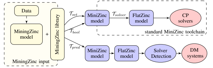
Figure 1: Overview of the MiningZinc toolchain
